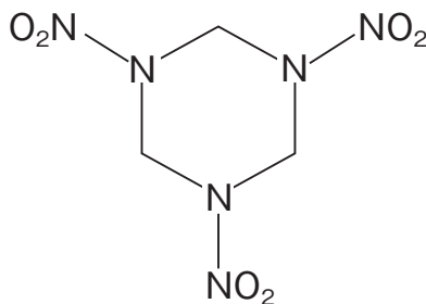
Figure 1 Chemical structure of RDX.
